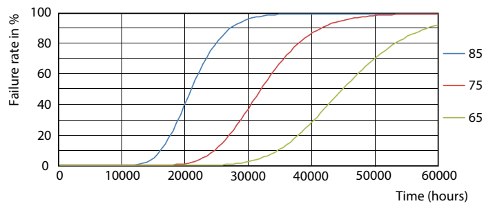
FailureRate
